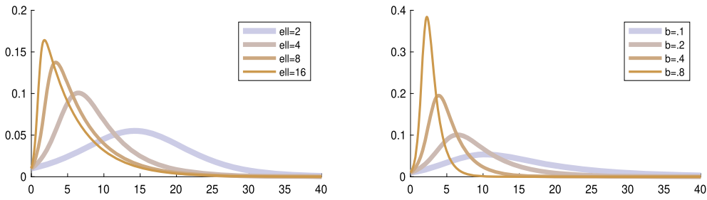
FIG. 3. Stationary solution for different values of \ell , with b = 0.2 (left), and for different values of b , with \ell = 4 (right). In all cases, \rho = -0.01, a = 1, \lambda = 1 .
