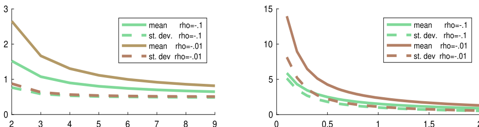
FIG. 4. Stationary mean and standard deviation for 2 \leq \ell \leq 9 , with b = 2, a = 1 (left) and for 0.1 \leq b \leq 2 , with \ell = 4, a = 1 (right).
