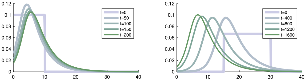
FIG. 2. Solution of (1.3) for initial condition \text{unif}[0, 10] (left) and \text{unif}[15, 30] (right) at different time instances, with \rho = -0.01, c_1 = 0.21, b = 0.2, \ell = 4, a = 1 .
